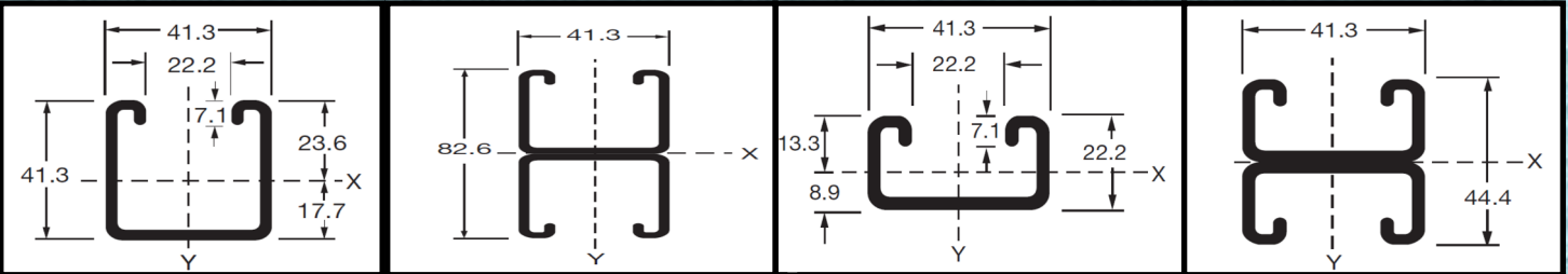
41.3mm x41.3mm Single and Double Solid
